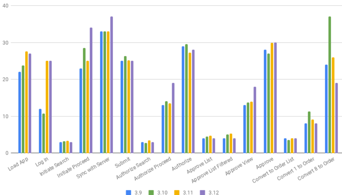
UI Performance: Loading times for versions 3.9 through 3.12
