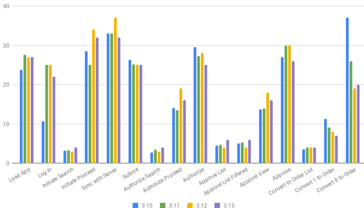
UI Performance: Loading times for versions 3.10 through 3.13
