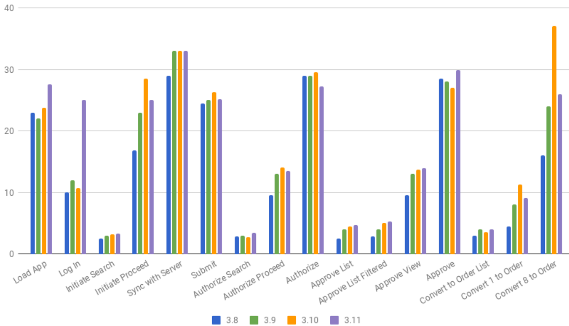
UI Performance: Loading times for versions 3.8 through 3.11
